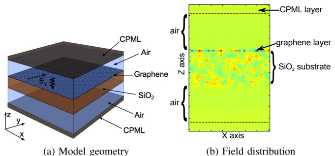
Fig. 1. (a) 3D EMC-FDTD model geometry. The wavy arrow denotes the direction of propagation of the wave, while the direction of the electric field is shown by the dotted arrow. The domain boundaries perpendicular to x and y are terminated by periodic boundary conditions. (b) Visualization of the spatial distribution of the electric field ( E_y ) stemming from the influence of the carriers in the graphene sheet and the charged impurities in the SiO 2 substrate at the start of the simulation.
