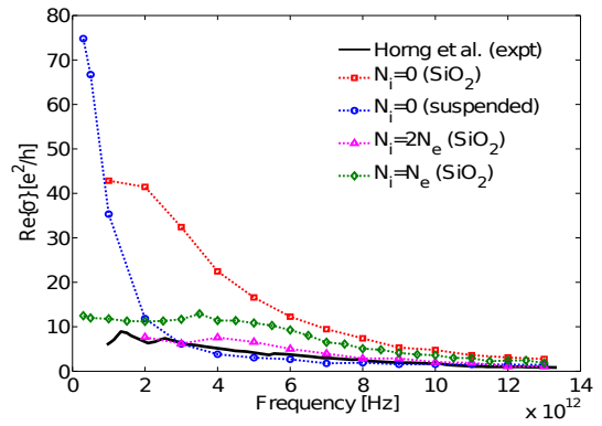
Fig. 3. The real part of the complex conductivity of graphene as a function of frequency at the carrier density of N_e = 6.3 \times 10^{12} \text{ cm}^{-2} , which is the same density for a gate voltage of 50 V in Ref. [6]. Blue circles denote suspended graphene without impurities, red squares denote graphene on \text{SiO}_2 substrate without impurities, green diamonds and pink triangles denote different impurity levels in supported graphene, and the black solid curve corresponds to the experimental data from Horng et al. (Ref. [6]). Good agreement with experimental data is found for impurity density exceeding the electron density twofold ( N_i = 2N_e .)
