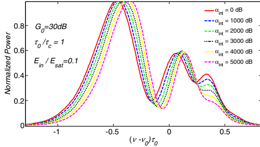
Fig. 4. The output pulse spectrum corresponding to the pulse shapes shown in Fig. 2. Medium loss causes a blue shift in spectrum and the gain recovery impact can be seen on the spectrum.
